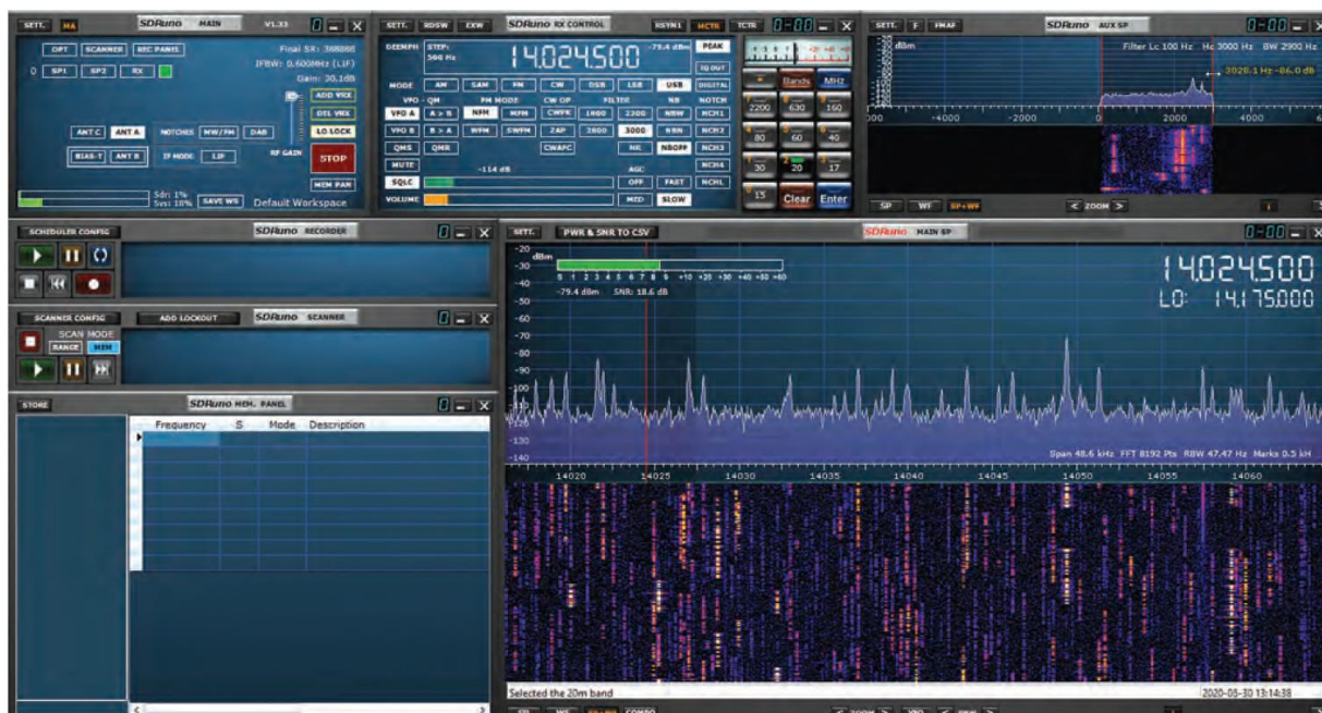
Rys. 4.1. Program SDRRuno
